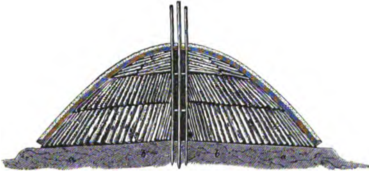
Fig. 311.—Section of charcoal-kiln.
